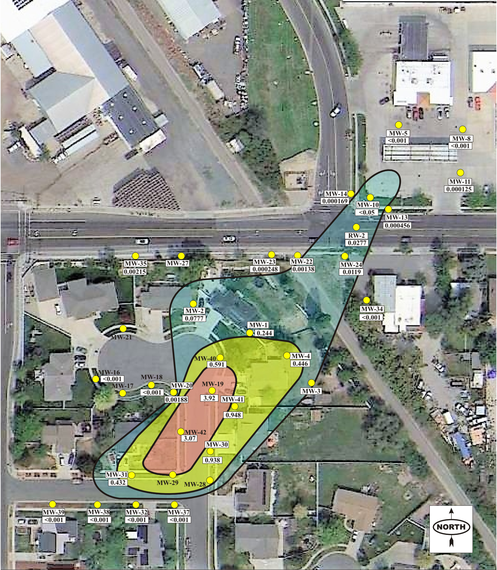
Triple Stop Chevron 1034 W Gentile Street Layton, Utah Figure 1 Dissolved Benzene January 2022
